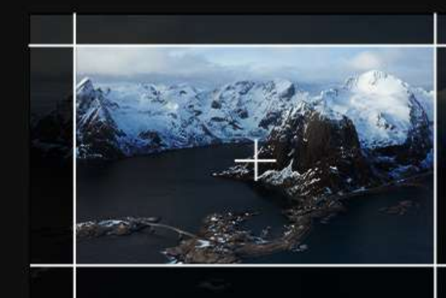
User Markers
